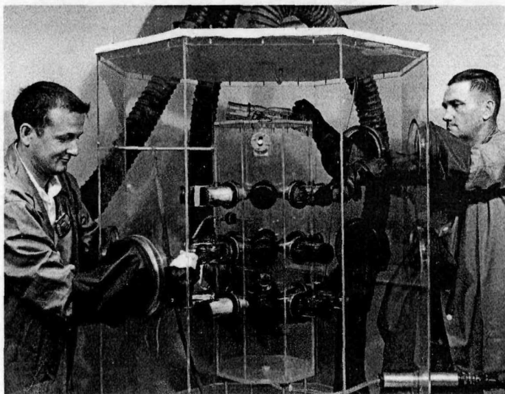
Studies of inhalation of radioactive materials are conducted in this specially constructed aerosol chamber. Soft drink bottles have been adapted to serve as animal holders.
